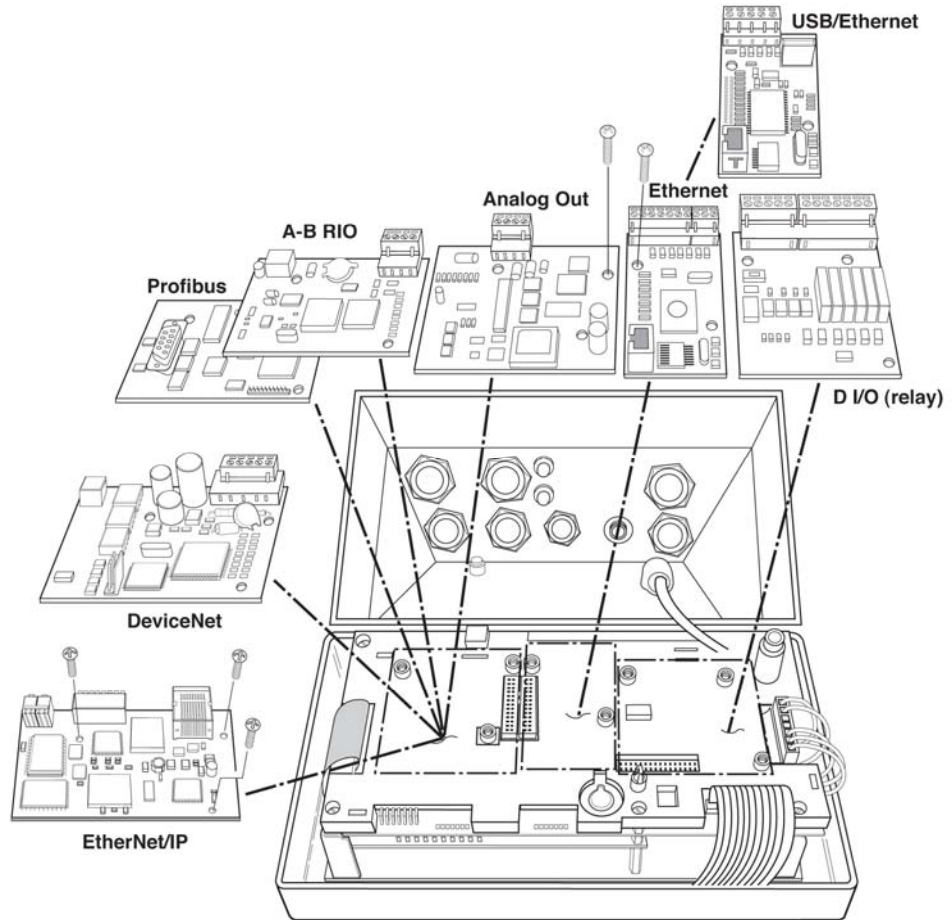
Figure 2-23: Option Locations for Harsh Enclosure
