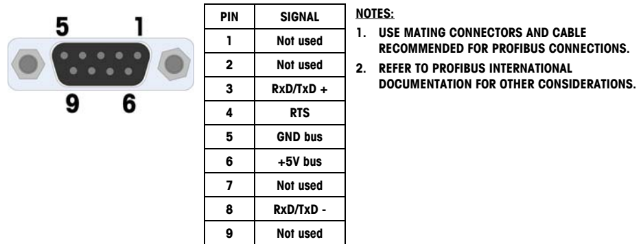
Figure 2-44: PROFIBUS Nine-Pin Connector Assignments
