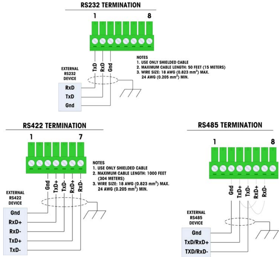
Figure 2-22: Sample COM1 Connections
