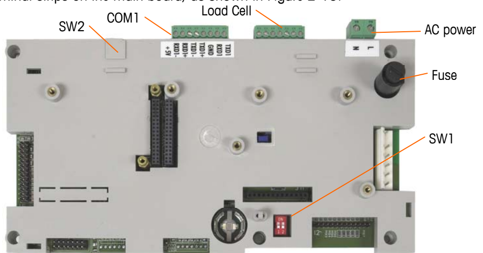
Figure 2-15: Analog Main Board in Harsh Enclosure
