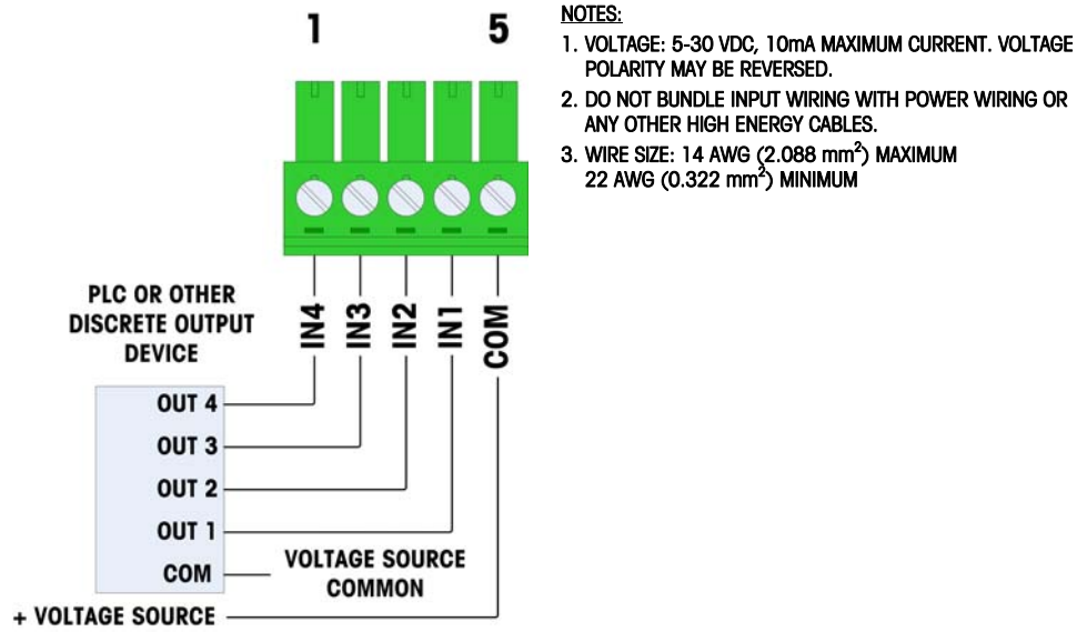
Figure 2-34: Passive Input Connections
