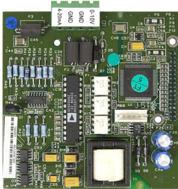
Figure 2-25: Analog Output Option Board
