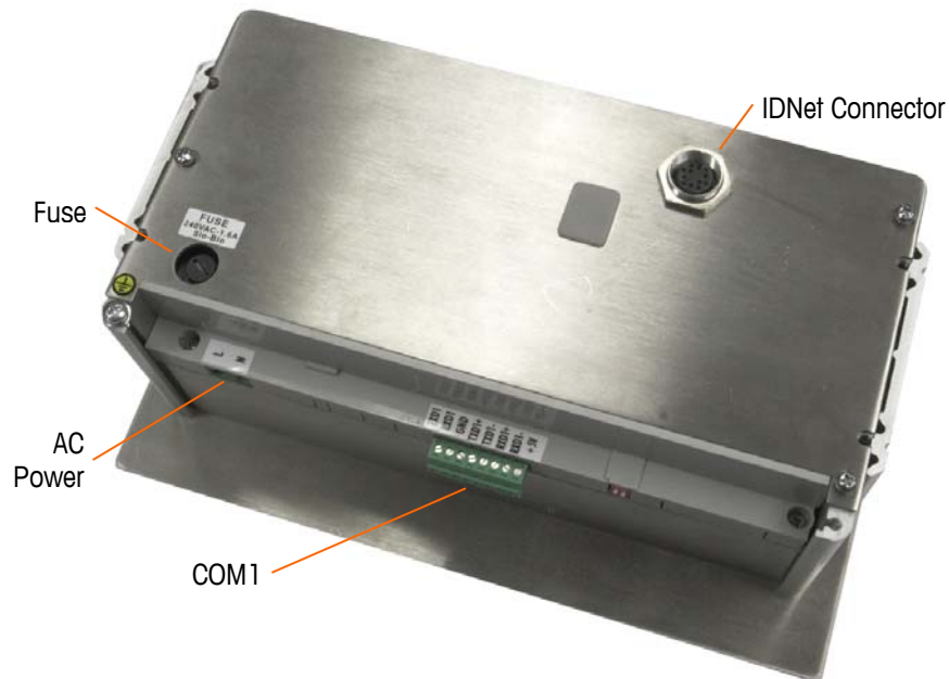
Figure 2-16: Panel Mount Enclosure Connections, including IDNet
