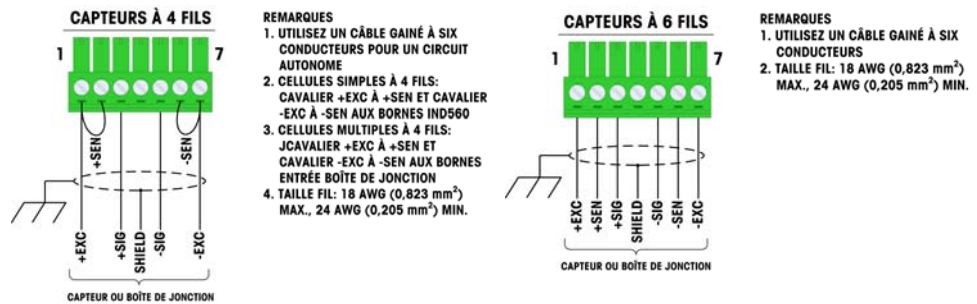
Figure 2-17 : Raccordements de cellule de pesage
