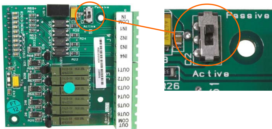
Figure 2-50: Location (l) and Switch Settings (r) for Relay Discrete I/O Switch
