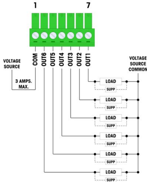
Figure 2-35: Relay Outputs
