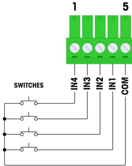
Figure 2-33: Active Input Connections
