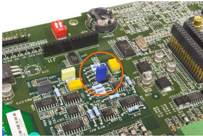
Figure 2-51: W1 Millivolt Jumper Location, Main PCB Uncovered
