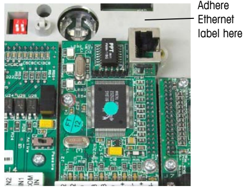
Figure 2-31: Ethernet Label Location for the Harsh Enclosure
