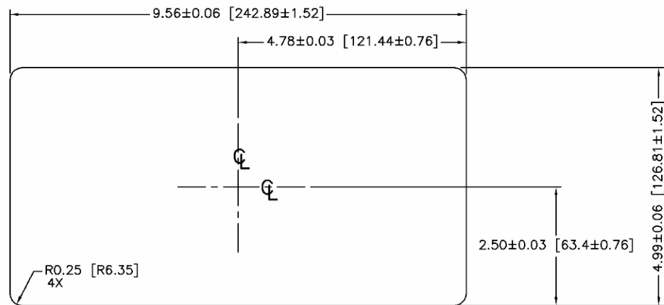
Figure 2-6: Panel Cutout Dimensions
