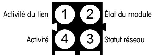
Figure 2-46: LED d'indication d'état Ethernet / IP
