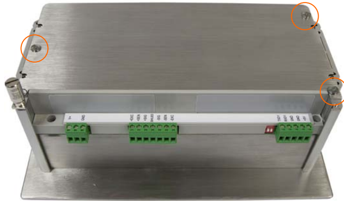
Figure 2-1: Opening the Panel-Mount Enclosure
