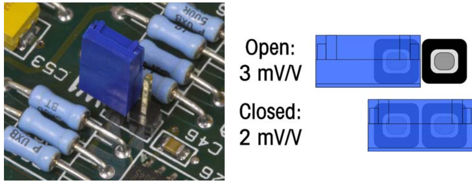
Figure 2-53: W1 Millivolt Jumper Settings
