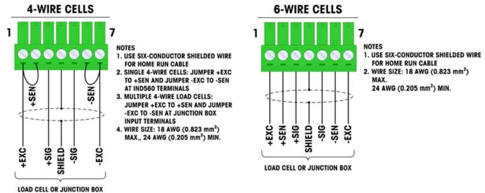
Figure 2-17: Load Cell Termination
