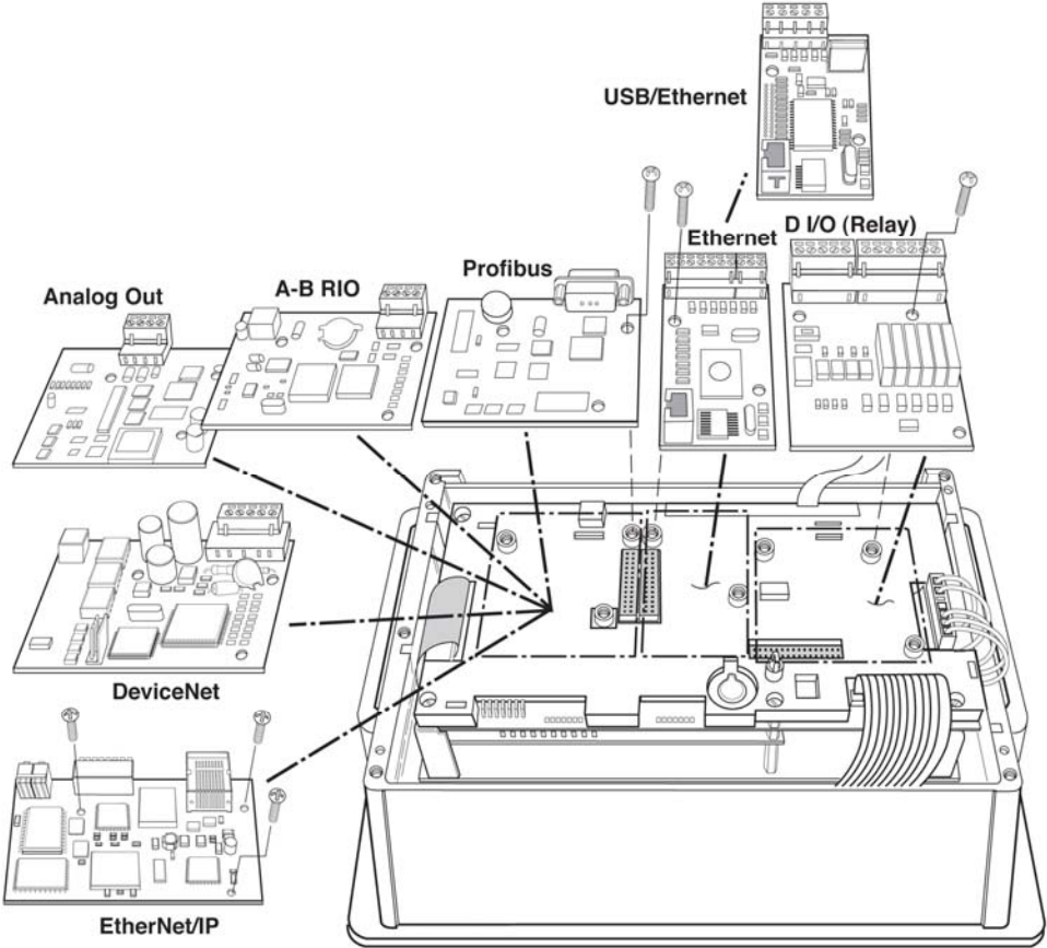
Figure 2-24: Option Locations for Panel-Mount Enclosure
