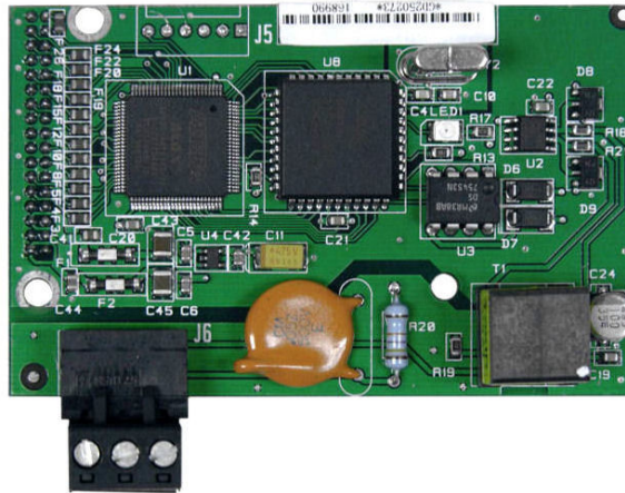
Figure 2-36: Option A–B RIO
