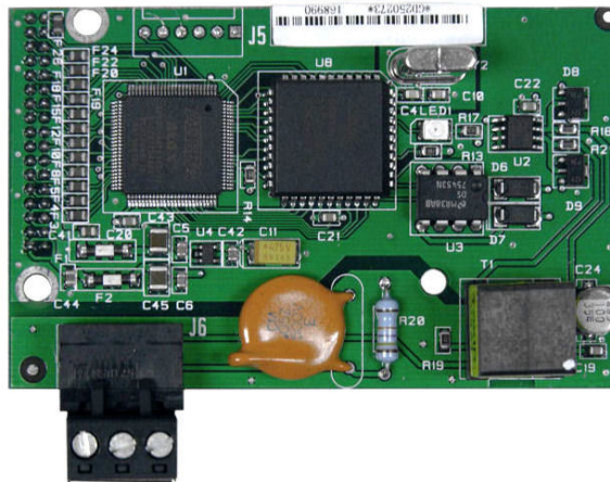
Figure 2-36: A-B RIO Option Board
