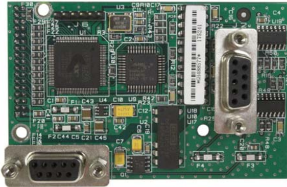
Figure 2-41: PROFIBUS Option Board, Harsh Enclosure
