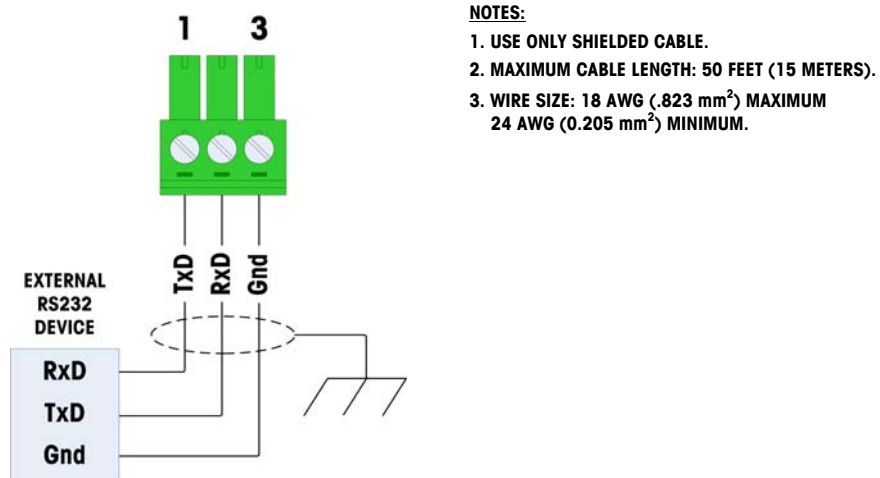
Figure 2-28: Wiring to COM2
