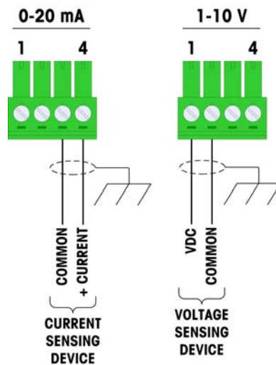
Figure 2-26: Wiring the Analog Output
