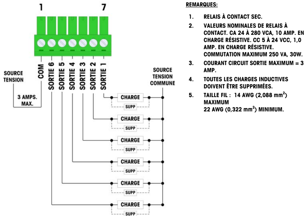
Figure 2-35: Sorties relais
