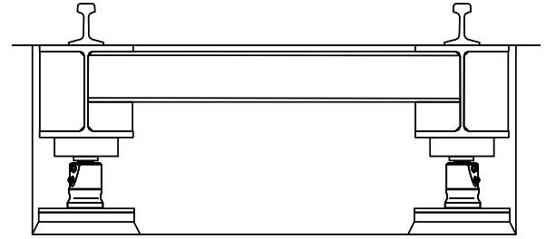
7260 Cross Section
