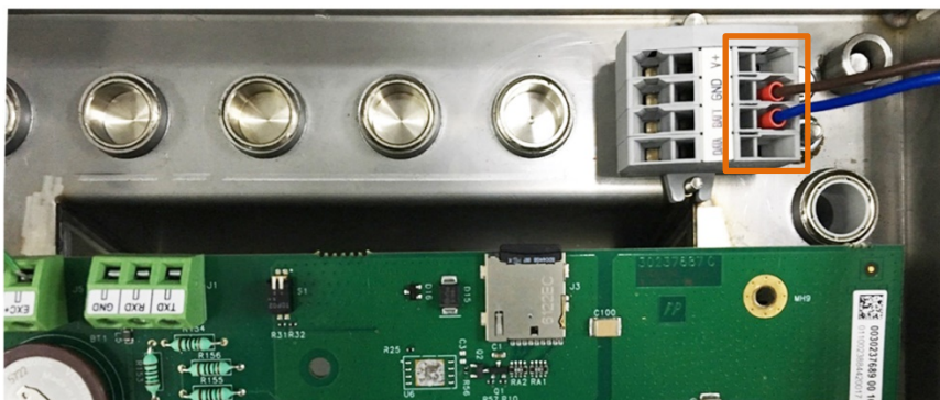
Figure 3-3: Wiring to the Terminal Connector
