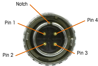
Figure 4-3: Battery Connector Pin Location
