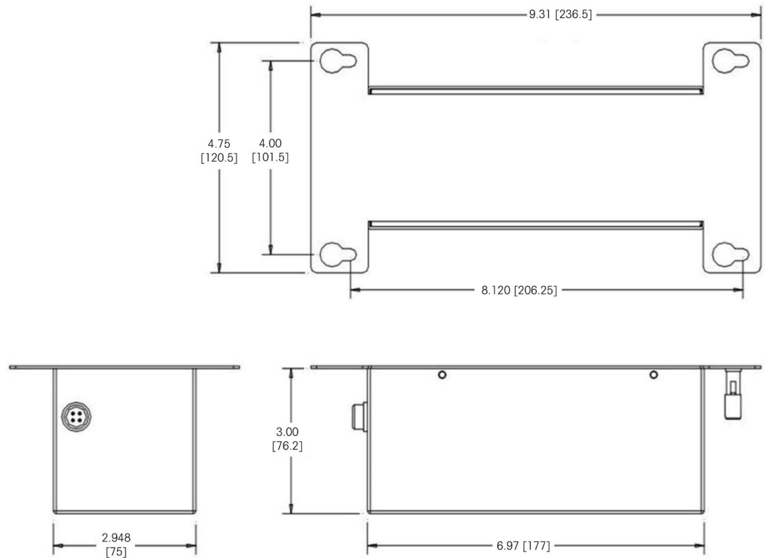
Figure 1-4: 64060625 Battery Pack General Dimensions
