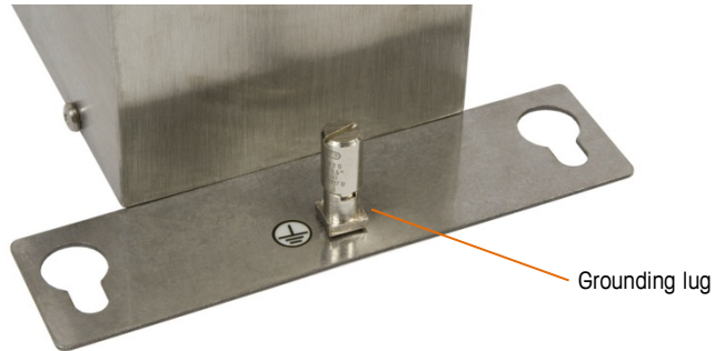
Figure 3-6: Grounding Lug
