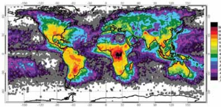
Lightning strikes an average of 8.6 million times per day globally. This world lightning map by NASA shows the geographic distribution of the strikes.
